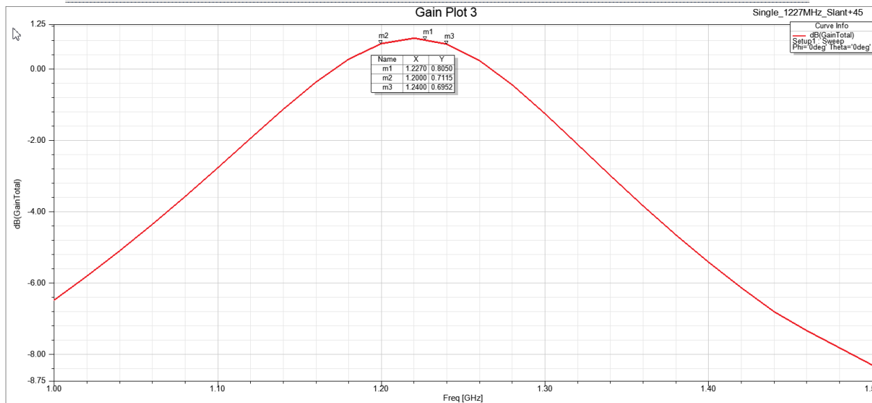
Rectangle Patch Slanted +45 Polarized Frequency: 1.227GHz
